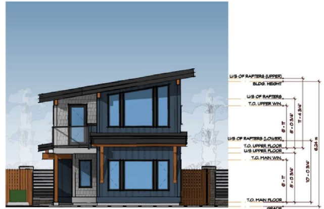
FRONT ELEVATION 3/16" = 1'-0"
