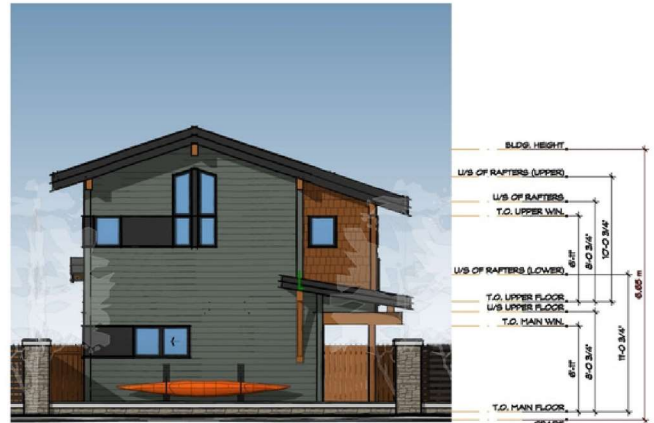
REAR ELEVATION 3/16" = 1'-0"
