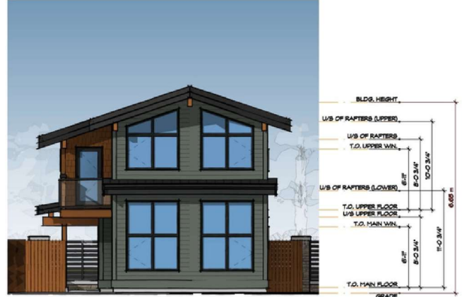
FRONT ELEVATION 3/16" = 1'-0"
