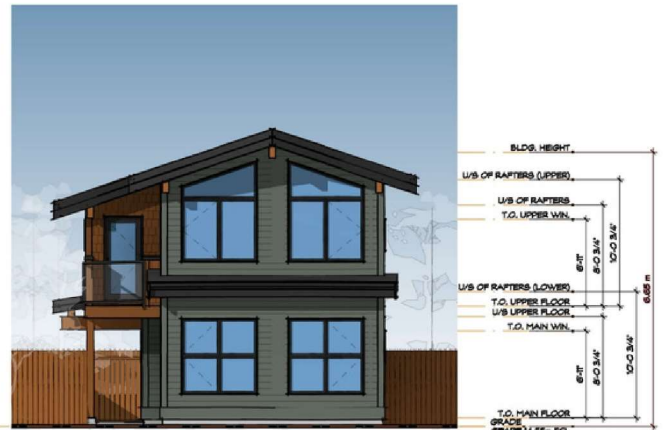
FRONT ELEVATION 3/16" = 1'-0"
