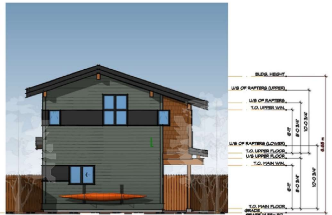
REAR ELEVATION 3/16" = 1'-0"
