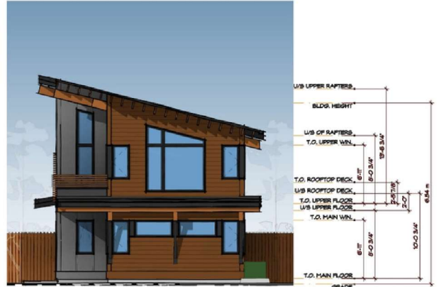
FRONT ELEVATION 3/16" = 1'-0"
