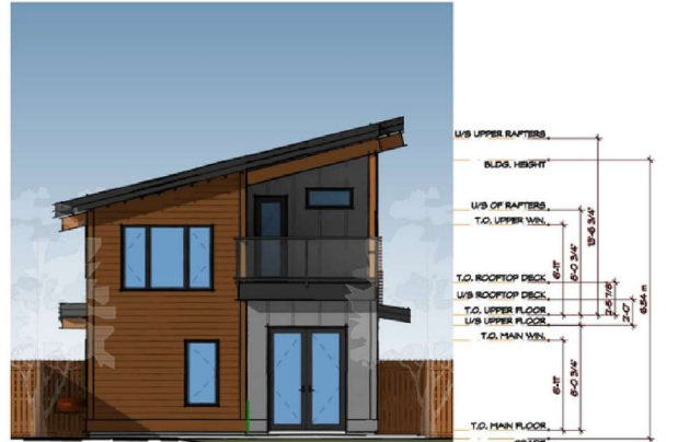
REAR ELEVATION 3/16" = 1'-0"
